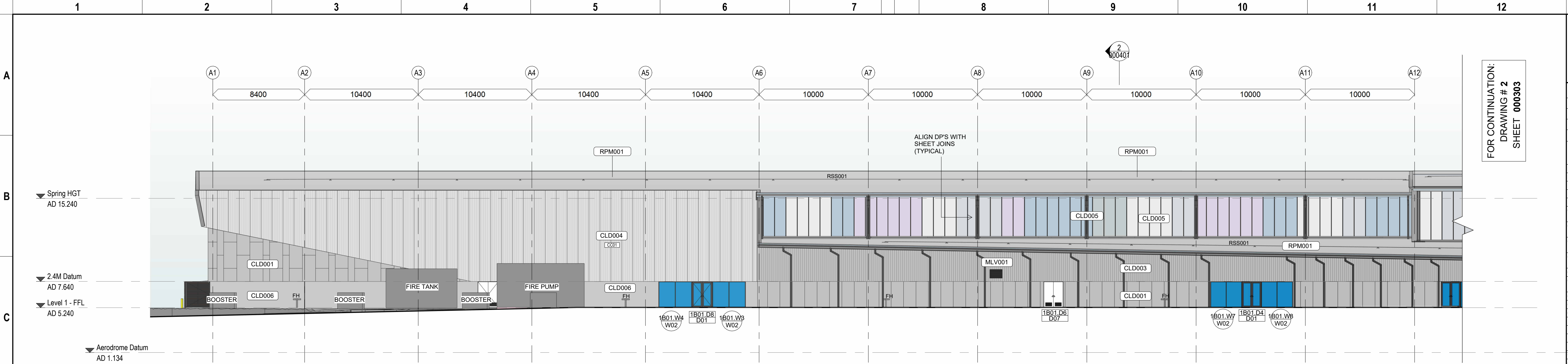
1 SOUTH EAST - PART A 1 : 200
